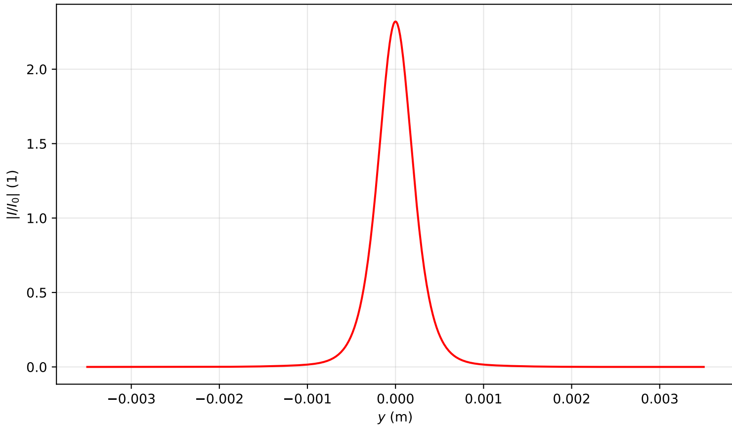
Intensity profile I(x=0, y, z=2.388)/I_0 , P_{in}=1.0P_{cr} , artificial time
